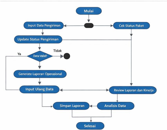
Gambar 2. Activity Diagram
