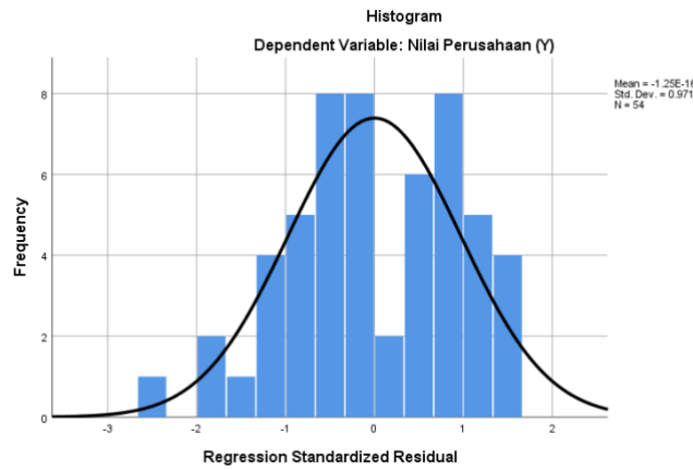
Gambar 2. Histogram
