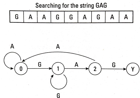
Gambar 2. Contoh algoritma Finite Automaton
