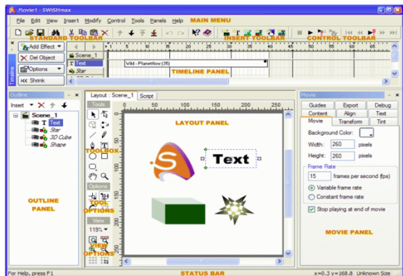
Gambar 5. Interface SwishMax
