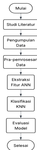
Gambar 1. Flowchart Penelitian
